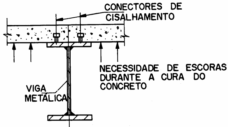
(A) LAJE FUNDIDA IN LOCO
